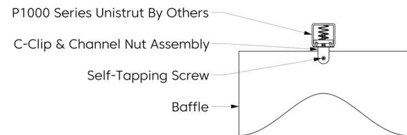
Threaded Rod To Unistrut
