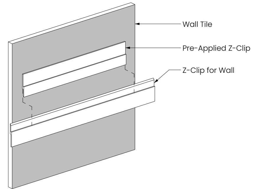
Z-Clip Mount
